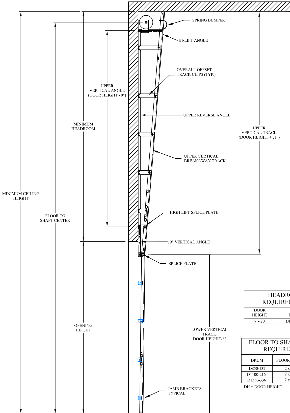
VERTICAL LIFT STANDARD 2" BRACKET MOUNT TRACK SET DETAIL
