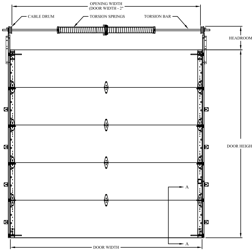
INTERIOR ELEVATION
