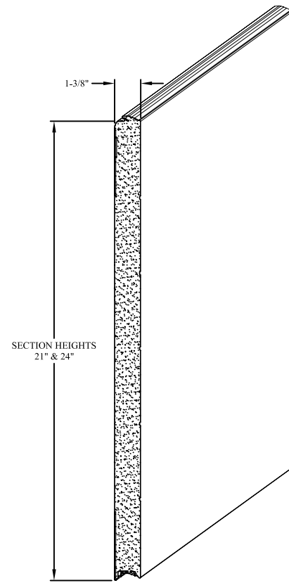
ISOMETRIC PROFILE
