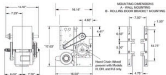
*For models with brakes add 2" (Standard on 3/4, optional on 1/2 HP)
